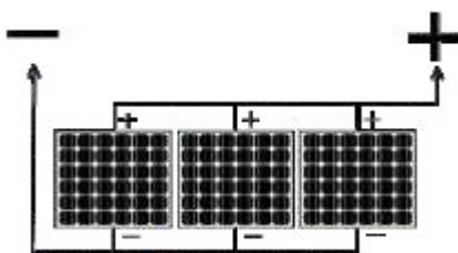
Parallel PV-Connector
